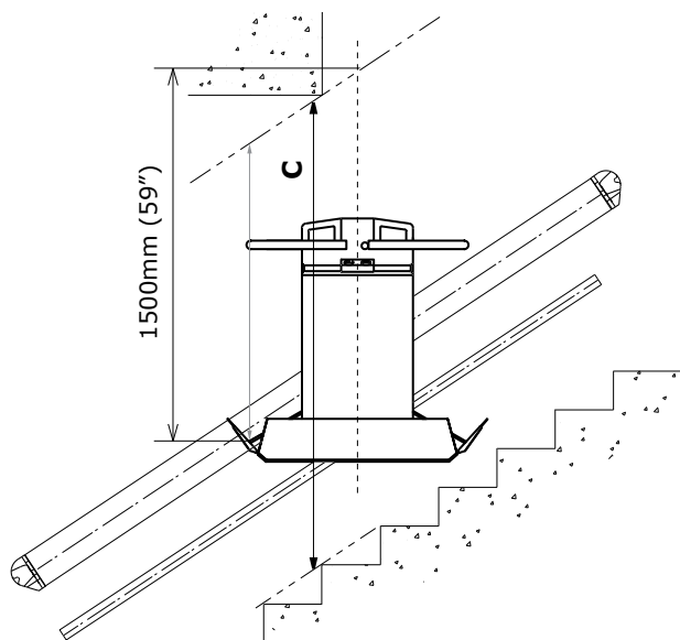
Overhead Clearances to meet Canadian Code Requirements (CSA B355-2000)
