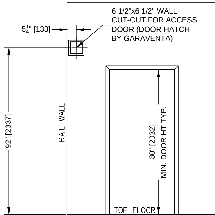
EMERG. LOWERING ACCESS DOOR LOCATION
