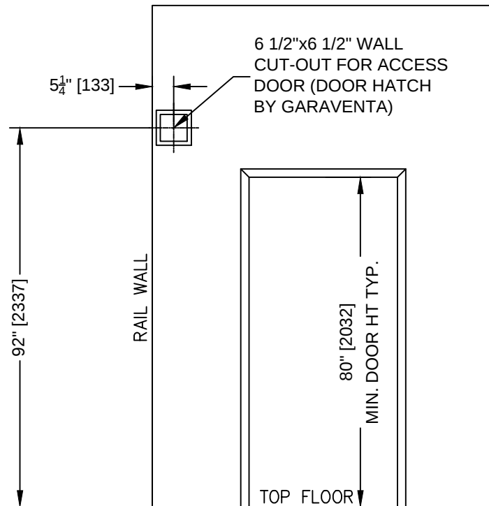
EMERG. LOWERING ACCESS DOOR LOCATION
