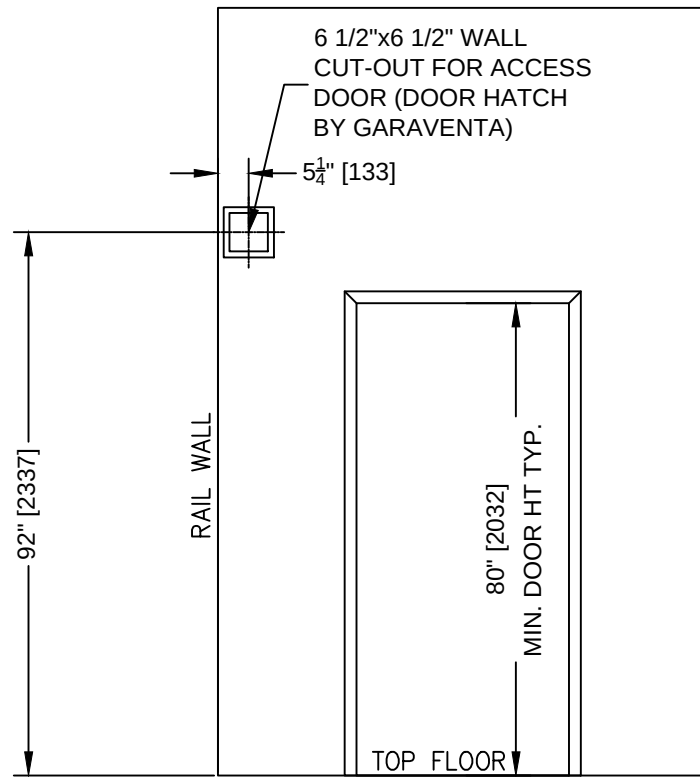
EMERG. LOWERING ACCESS DOOR LOCATION
